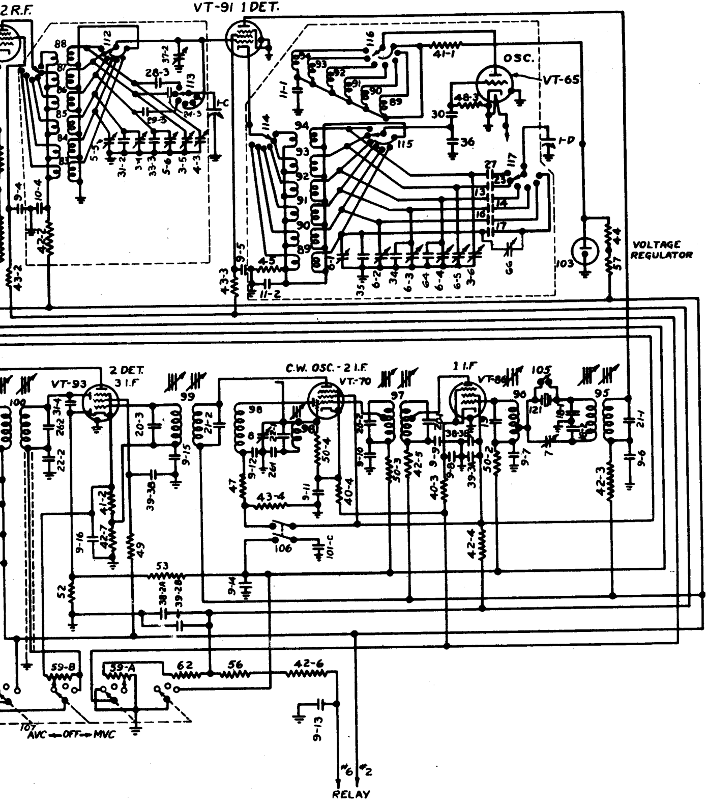
Figure 39 — Radio Receiver BC-348-O or BC-348-S, Schematic Circuit Diagram
