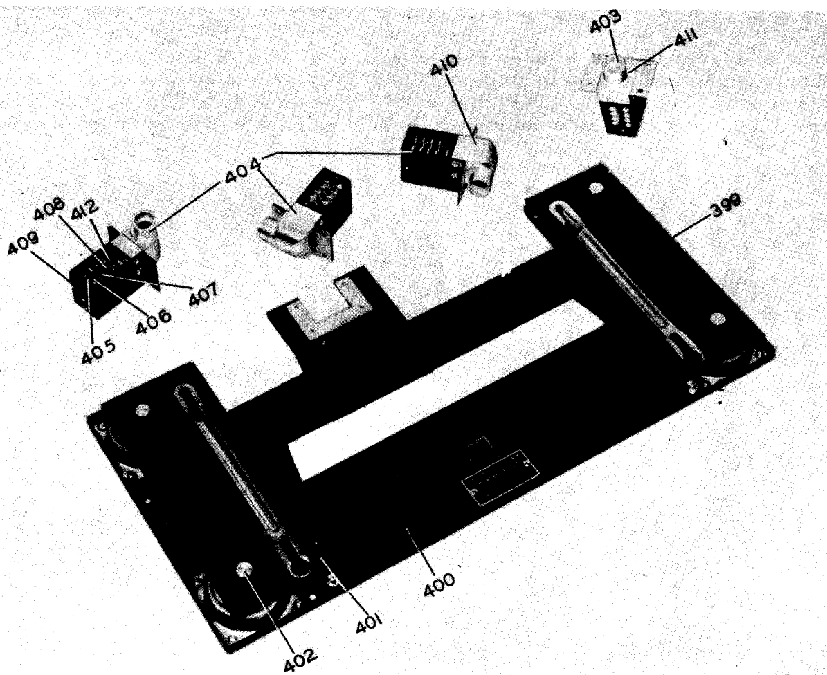
Figure 5 — Mounting and Plugs PL-P103 and PL-Q103
